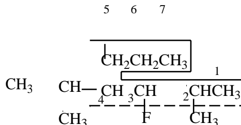
3-fluoro-4-isopropyl-2-methylheptane
