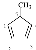
5-methylcyclopenta-1,3-diene
