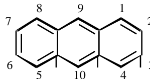
anthracene
