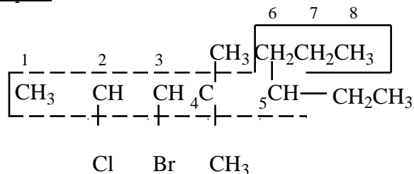
3-bromo-2-chloro-5-ethyl-4,4-dimethyloctane
