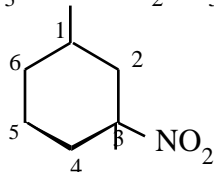
1- sec -butyl-3-nitrocyclohexane (numbering determined by the alphabetical order of substituents)
