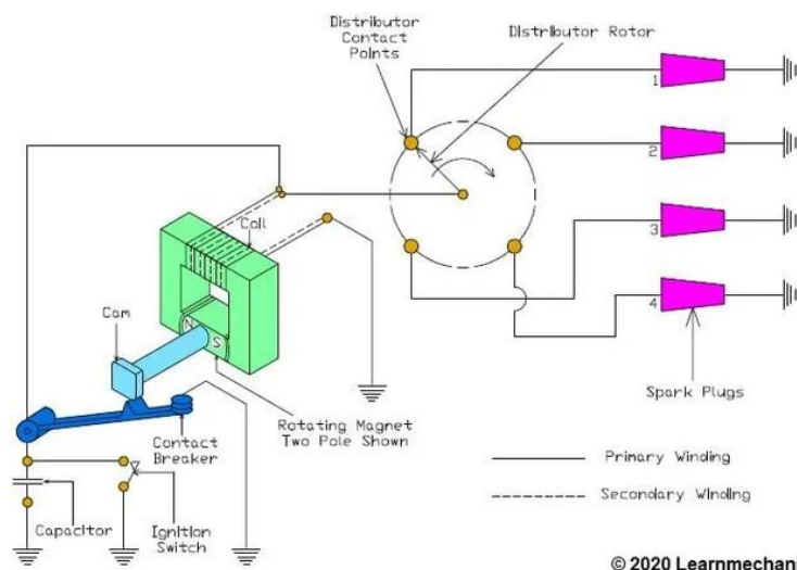
Magneto Ignition System
