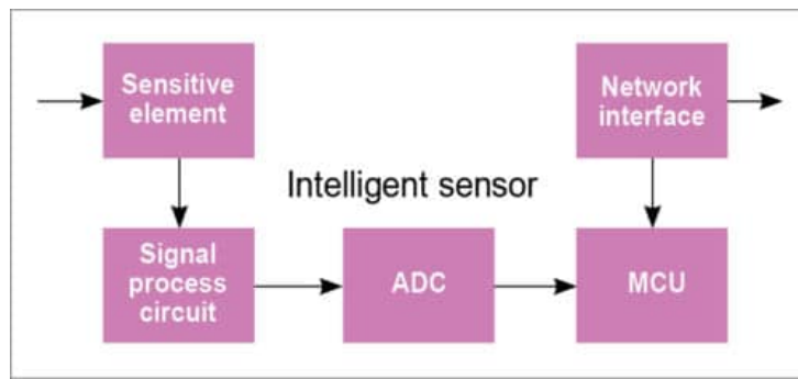
Fig. 1: Intelligent sensor structure (Courtesy: www.mdpi.com )
