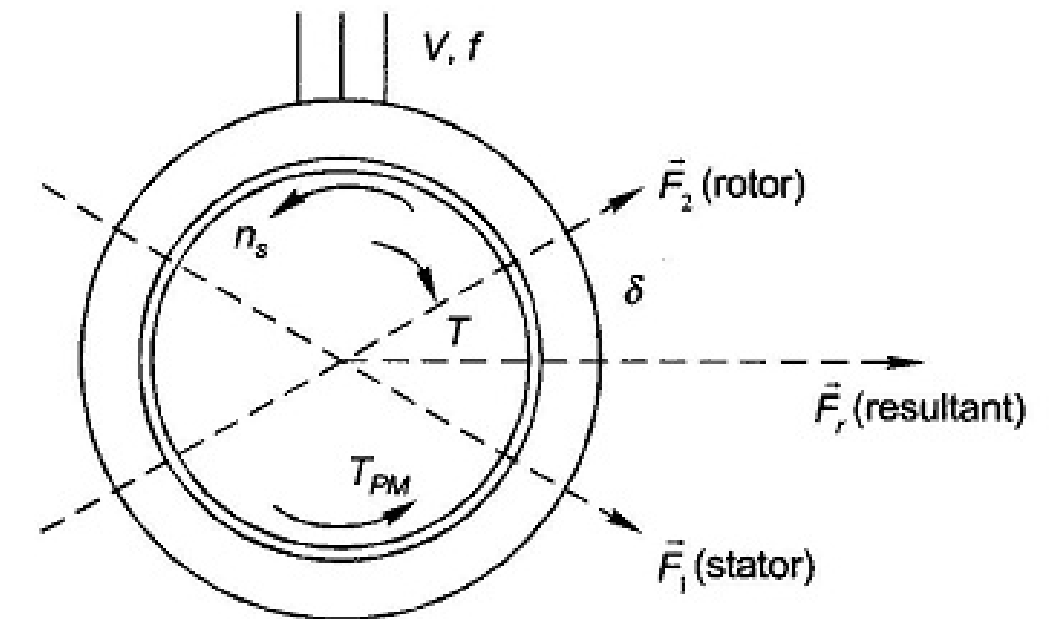
Torque production in synchronous machine (generating)
