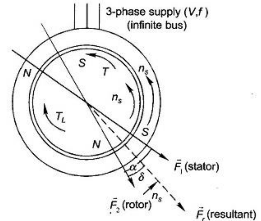
Torque production in synchronous machine (motoring)
