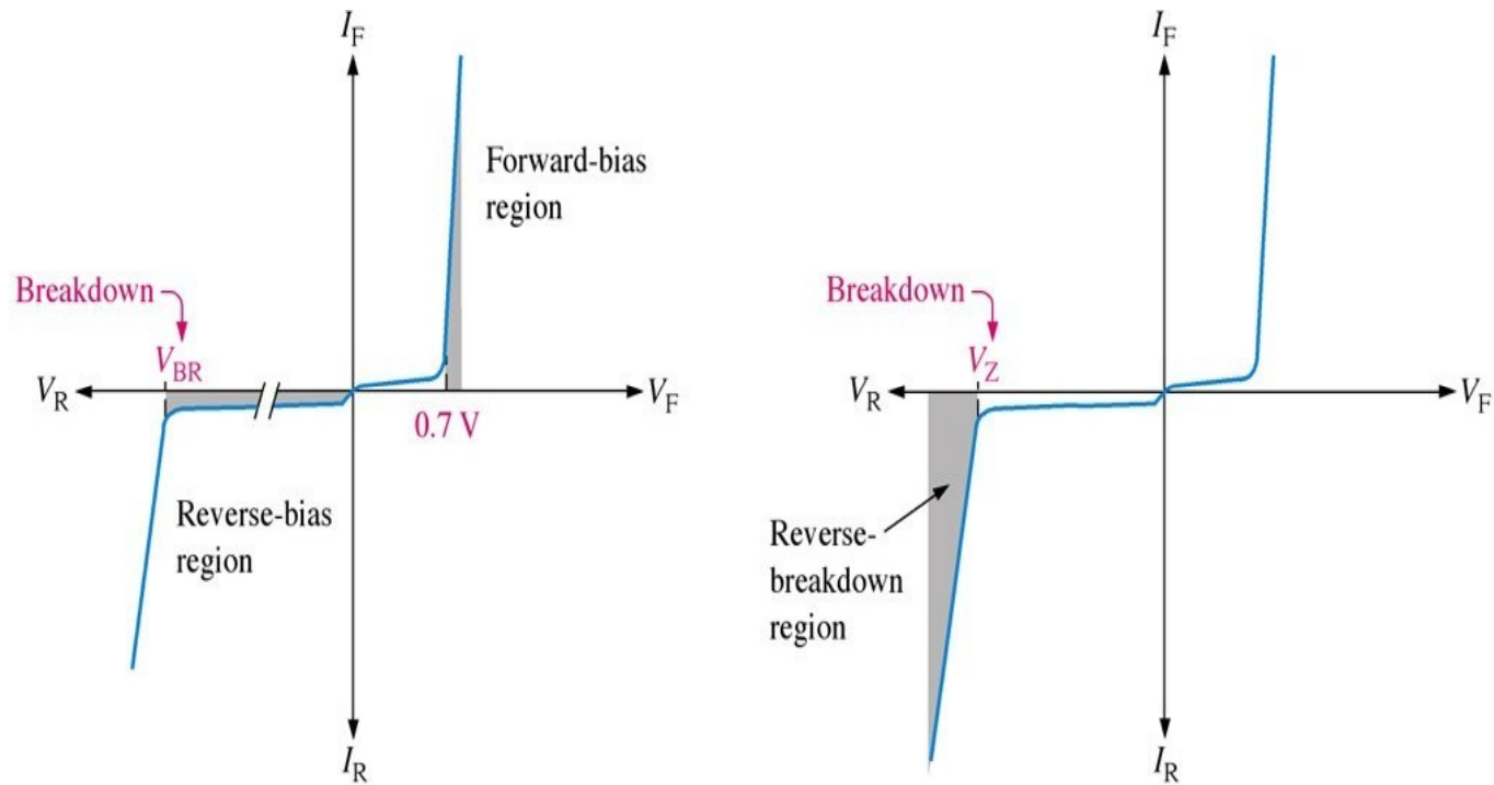
(a) The normal operating regions for a rectifier diode are shown as shaded areas.
