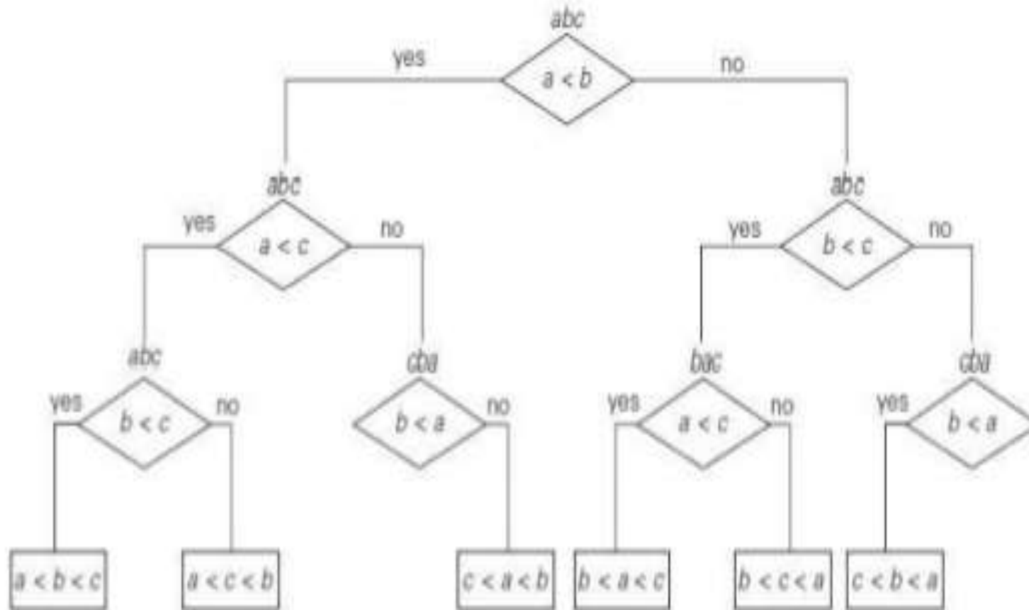
FIGURE 11.2 Decision tree for the tree-element selection sort. A triple above a node indicates the state of the array being sorted. Note two redundant comparisons b < a with a single possible outcome because of the results of some previously made comparisons.
