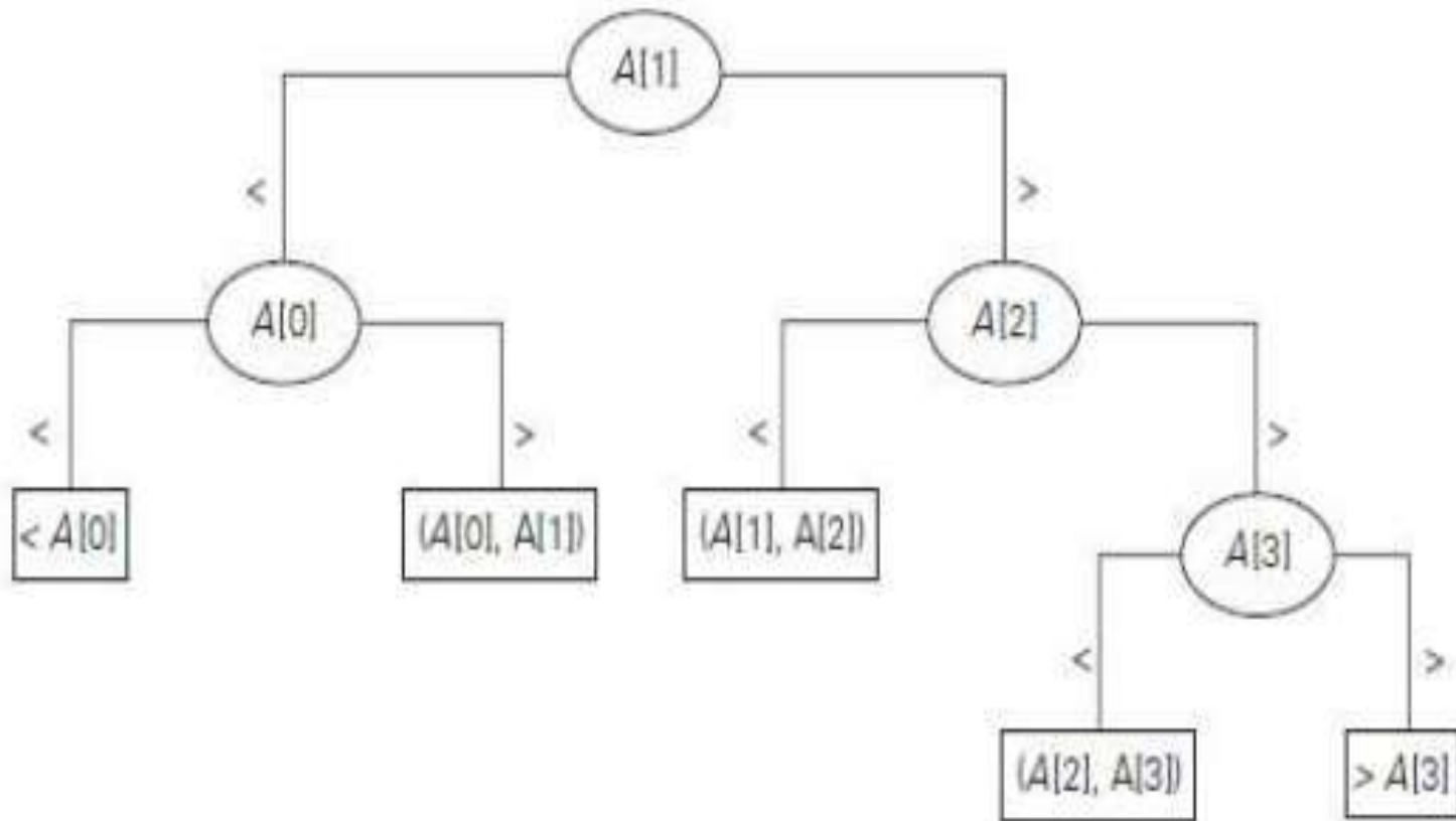
FIGURE 11.5 Binary decision tree for binary search in a four-element array.
