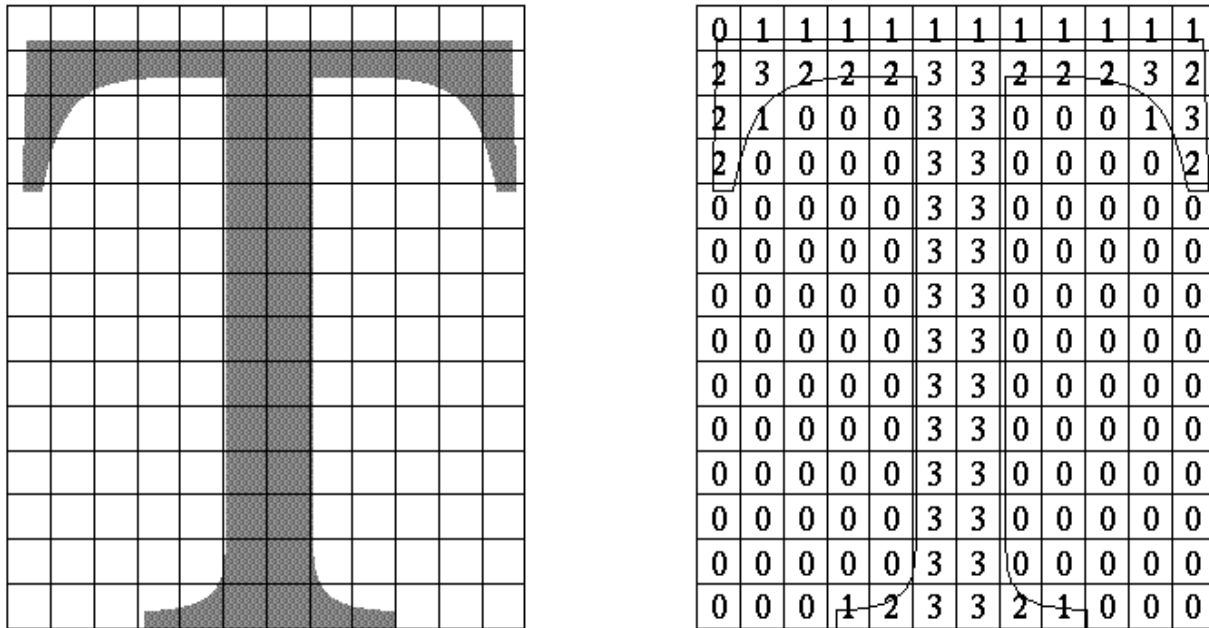
Figure 14-1 : Antialiased Characters
