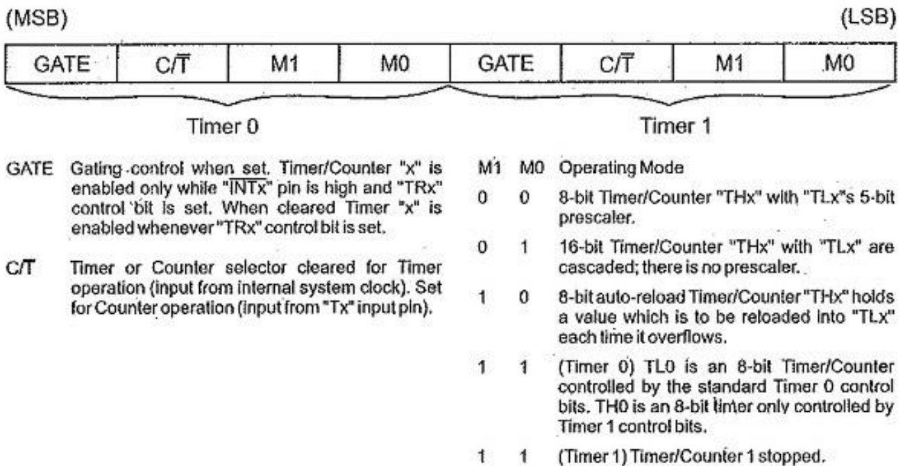
Figure 5.1.2 TMOD Register
